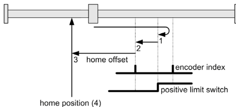
Figure 5-14 Homing Method 2
