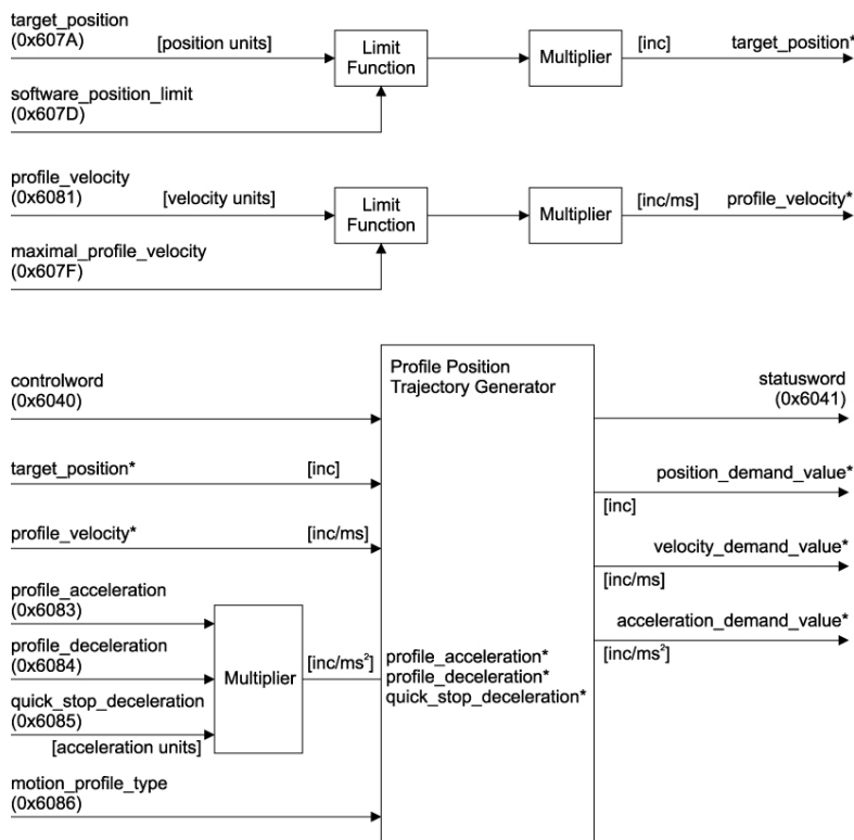
Figure 5-6 Profile Position Mode – Block Diagram
