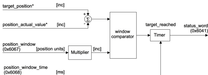
Figure 5-7 Profile Position Mode – Velocity Window
