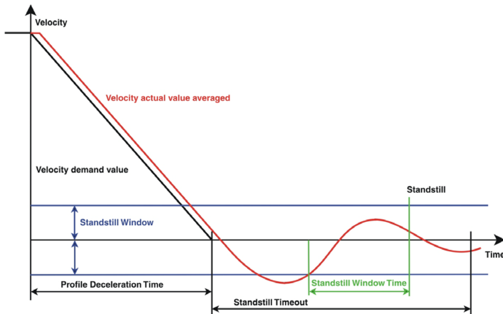
Figure 8-78 Standstill Window
