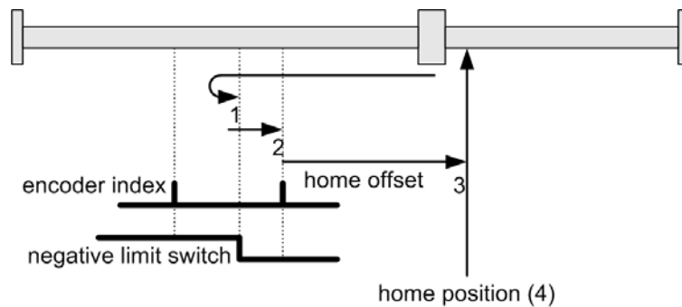
Figure 5-13 Homing Method 1
