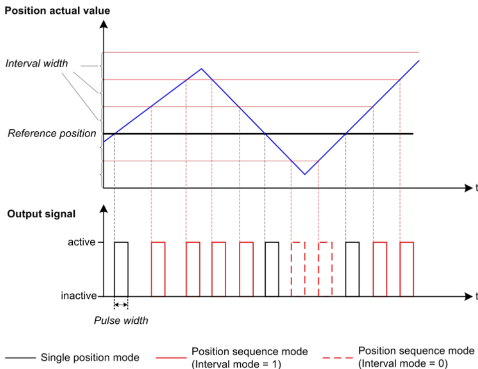
Figure 8-76 Position Compare – Overview
